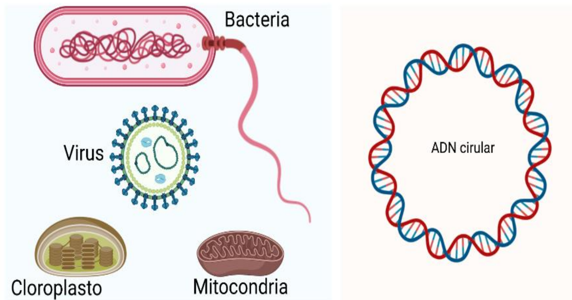
Figura 57 ADN circular
